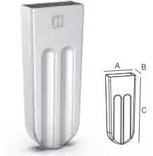
HY-C024 A:42.7mm B:19.3mm C:110mm ML/CC:70 B12/B14/B18/B22/B24 B26/B28
