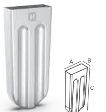
HY-C030 A:47.5mm B:19mm C:110mm ML/CC:71 B12/B24/B26
