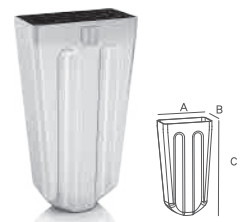
HY-C019 A:35mm B:18mm C:67mm ML/CC:32 B12/B14/B18/B22/B24 B26/B28
