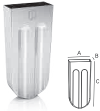
HY-C015 A:43mm B:19mm C:96mm ML/CC:63 B12/B14/B18/B22/B24 B26/B28
